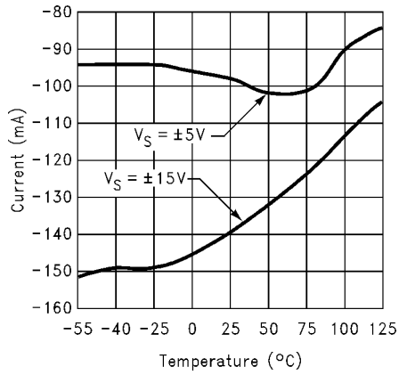
Short Circuit Current vs. Temperature (Sinking)
