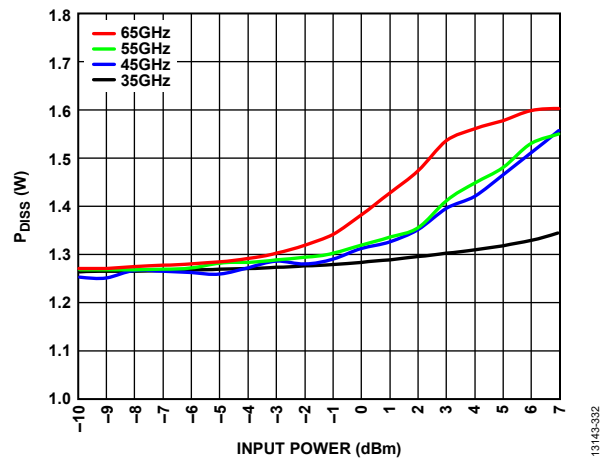
Figure 32. Power Dissipation ( P_{DISS} ) vs. Input Power at 85°C for Various Frequencies
