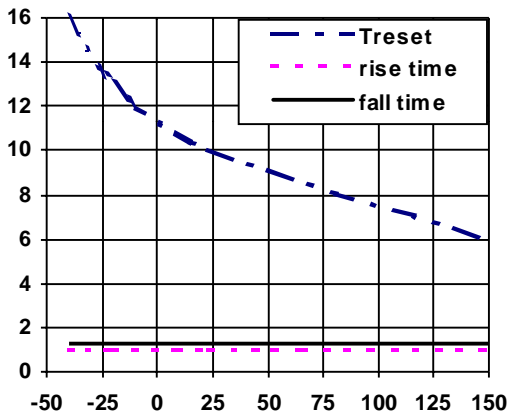
Figure 19 - Turn-on, Turn-off, and Treset (ns) Vs Tjunction (°C)
