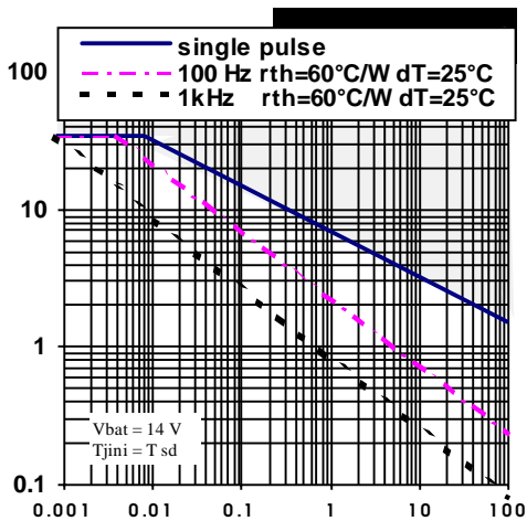
Figure 15 - Iclamp (A) Vs Inductive Load (mH)
