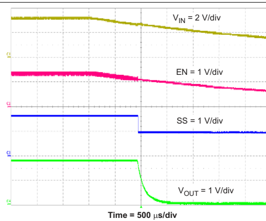
Figure 41. Transient Response
