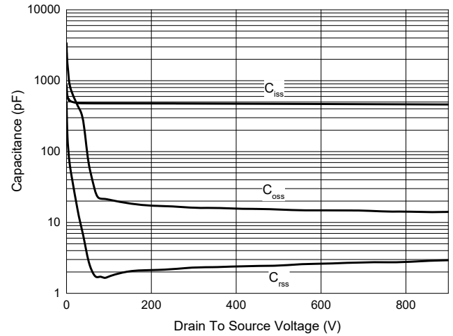
Fig. 8 - Capacitance Characteristics
