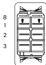
BOTTOM VIEW TERMINAL ARRANGEMENT 8 TERMINAL BASE
