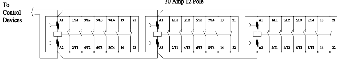
Wiring Diagram Class LE 30 Amp 12 Pole
