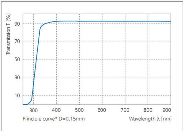
Figure 42. Transmission Characteristics of the Glass Lid
