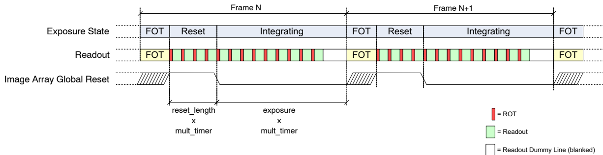
Figure 19. Integration Control for (Pipelined) Global Shutter Mode (Master)
