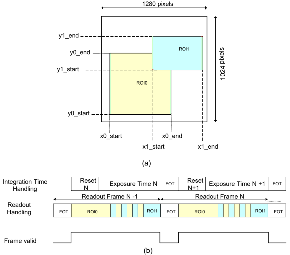
Figure 36. CMOS Mode: Frame Format to Read Out Image Data
