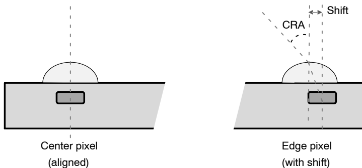
Figure 6. Principles of Microlens Shift. The Center Axes of the Microlens and the Photodiode Coincide for the Center Pixels. For the Edge Pixels, there is a Shift between the Axes of the Microlens and the Photodiode causing a Peak Response Incidence Angle (CRA) that deviates from the Normal of the Pixel Array.
