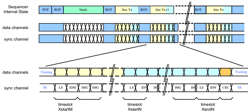
Figure 30. LVDS Mode: Time Line Showing the Readout of Two Overlapping Windows
