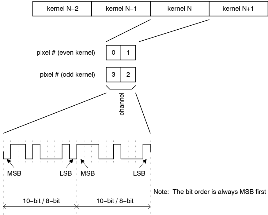
Figure 32. P1-SN/SE/FN: Data Output Order when Subsampling is Disabled
