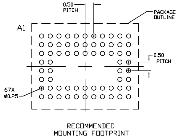
Figure 41. Package Drawing for the ODCSP67 Package
