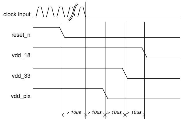
Figure 15. Power Down Sequence
