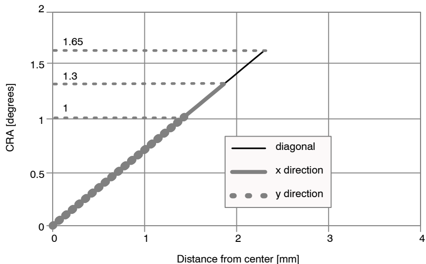
Figure 7. Variation of Peak Responsivity Angle (CRA) as a Function of Distance from the Center of the Array
