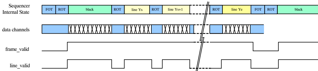
Figure 35. CMOS Mode: Frame Timing Indication
