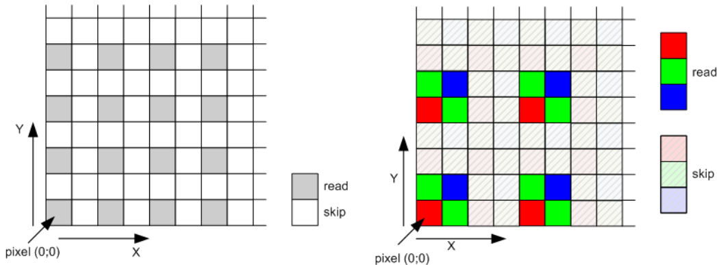
Figure 25. Subsampling Scheme for Monochrome and Color Sensors
