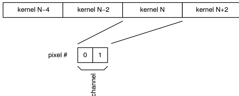
Figure 39. CMOS Mode: Data Output Order with Subsampling on a Color Sensor
