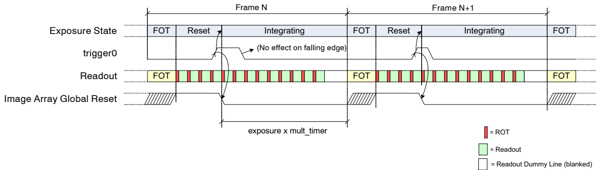
Figure 20. Exposure Time Control in Triggered Shutter Mode (Master)
