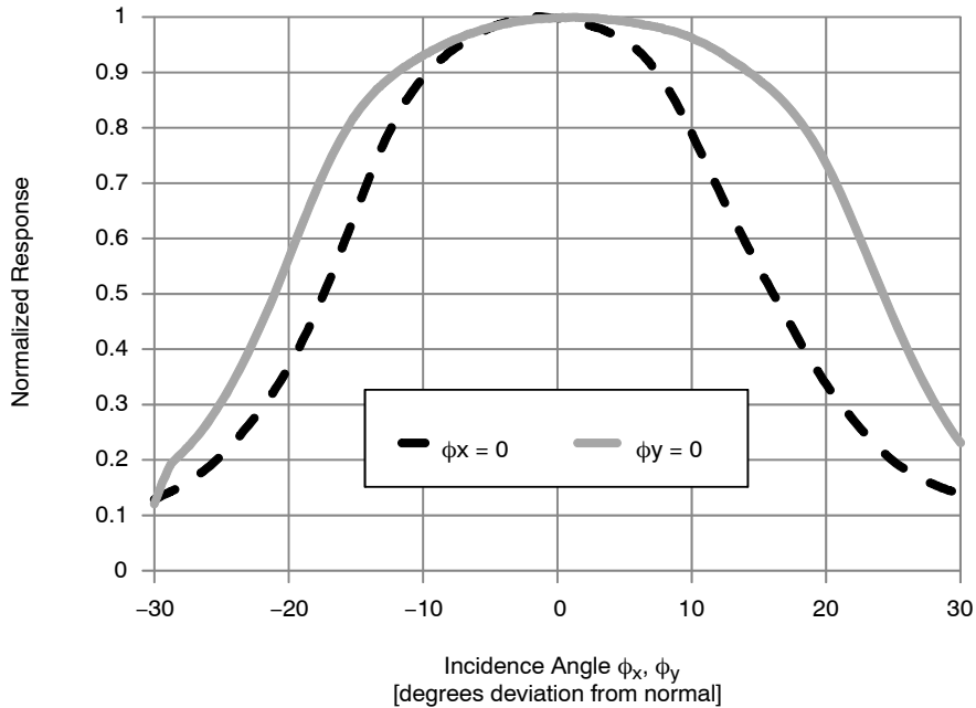
Figure 4. Central Pixel Photoresponse to a Fixed Optical Power with Incidence Angle varied along \phi_x and \phi_y . Note that the Photoresponse peaks near Normal Incidence for Center Pixels.
