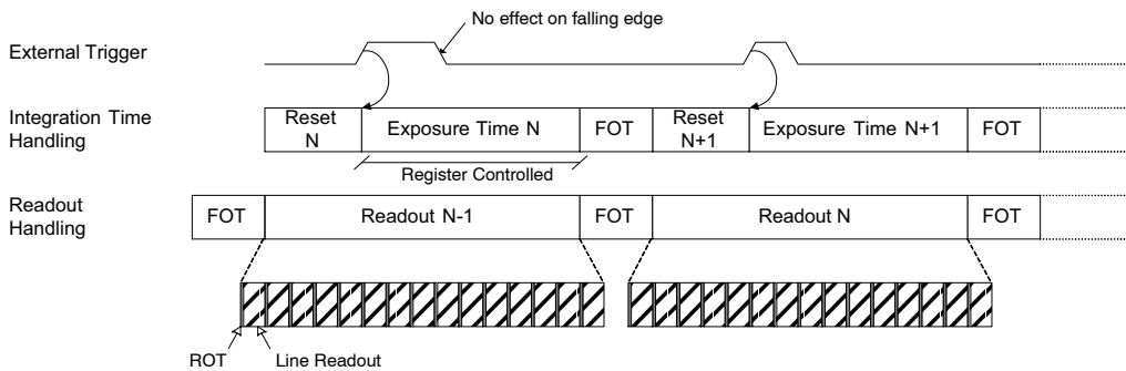
Figure 12. Triggered Shutter Operated in Master Mode
