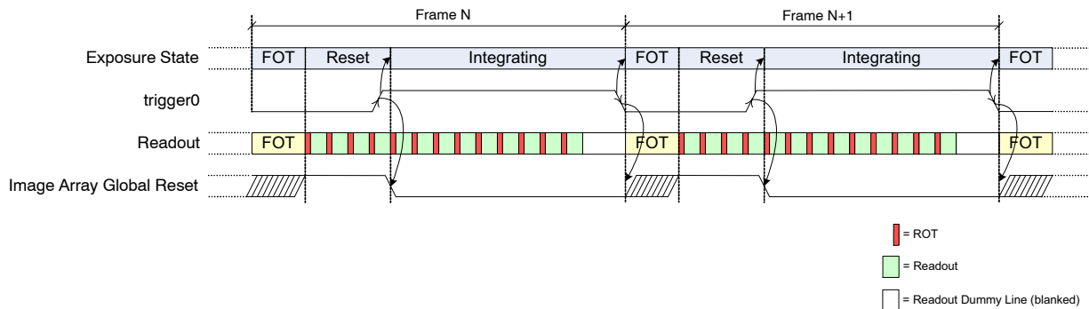
Figure 21. Exposure Time Control in Global-Slave Mode
