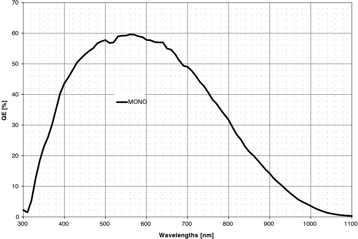
Figure 3. Quantum Efficiency Curve for Mono Sensor
