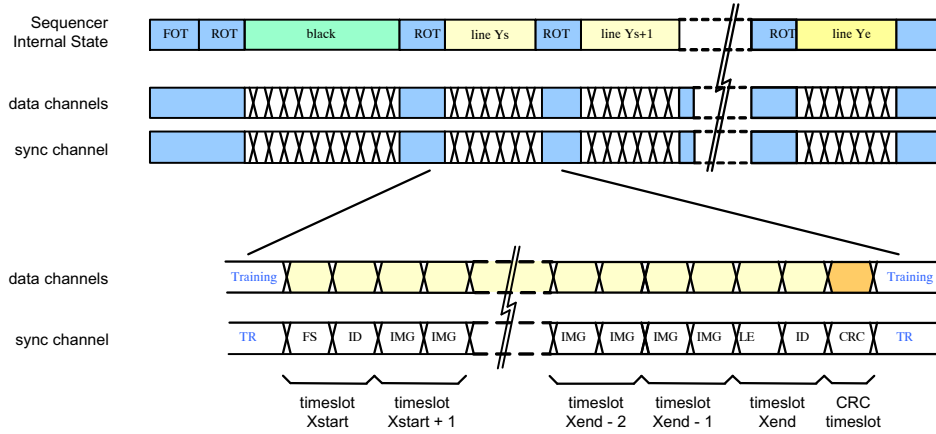
Figure 29. LVDS Mode: Time Line for Single Window Readout (at the start of a frame)
