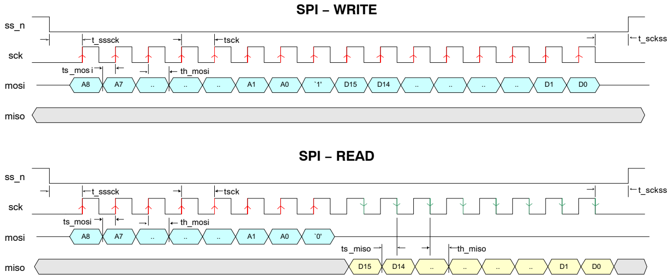
Figure 18. SPI Read and Write Timing Diagram
