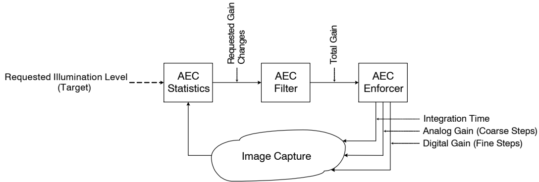
Figure 26. Automatic Exposure Control Loop
