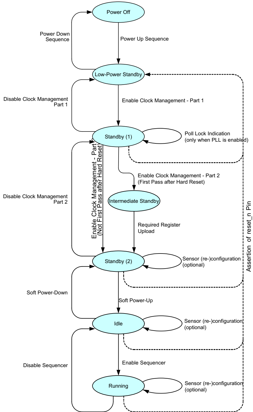
Figure 13. Sensor Operation Flowchart
