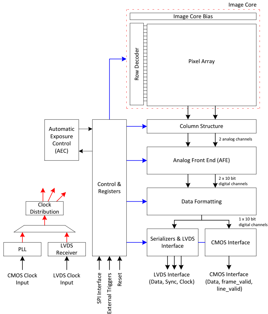
Figure 8. Block Diagram
