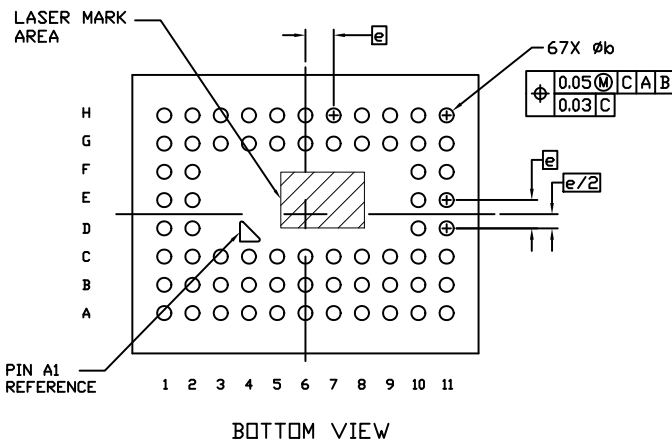
Figure 41. Package Drawing for the ODCSP67 Package
