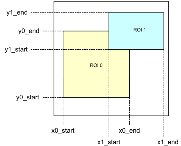
Figure 23. Overlapping Multiple Window Configuration
