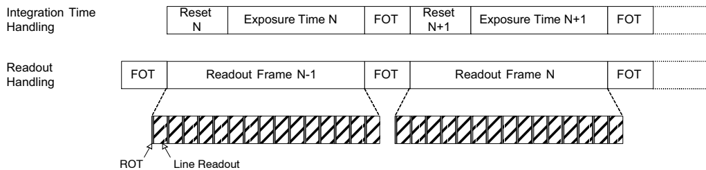
Figure 10. Integration and Readout for Pipelined Shutter
