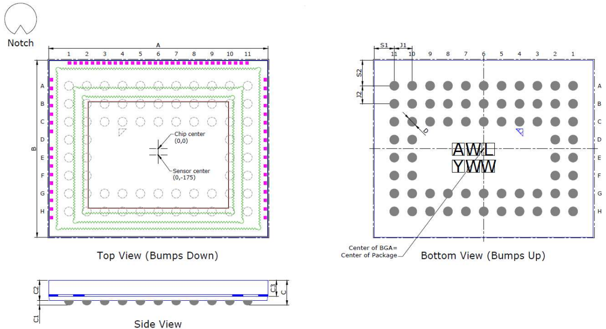
Figure 40. Mechanical Diagram
