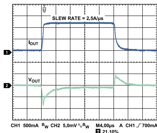
Figure 32. Load Transient Response, I_{LOAD} = 100\text{ mA} to 1.2\text{ A} , V_{OUT} = 3.3\text{ V} , V_{IN} = 4.0\text{ V} , Channel 1 = I_{OUT} , Channel 2 = V_{OUT}
