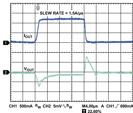
Figure 33. Load Transient Response, I_{LOAD} = 100\text{ mA} to 1.2\text{ A} , V_{OUT} = 3.3\text{ V} , V_{IN} = 4.0\text{ V} , C_{OUT} = 22\text{ }\mu\text{F} , Channel 1 = I_{OUT} , Channel 2 = V_{OUT}
