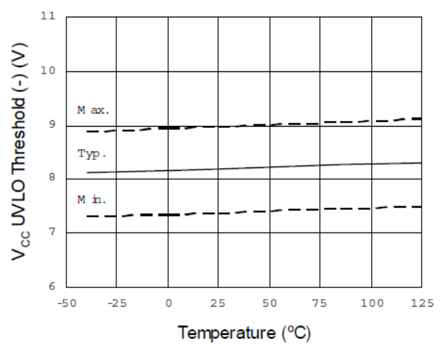
Figure 18. V CC Undervoltage Threshold (-) vs. Temperature
