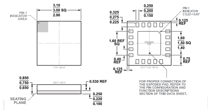
Figure 26. 20-Terminal Land Grid Array [LGA] 3 mm × 3 mm Body and 0.75 mm Package Height (CC-20-9) Dimensions shown in millimeters
