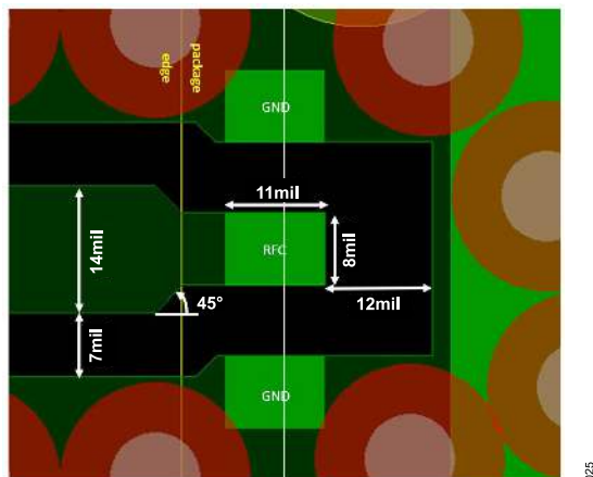
Figure 25. Recommended RF Pin Transitions
