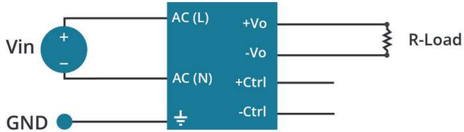
Figure 2 Remote Control Applications Circuit
