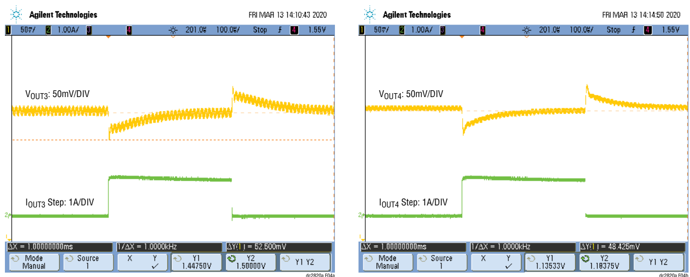
Figure 4. 12V IN Measured V_{OUT3} = 1.5V and V_{OUT4} = 1.2V Load Transient Responses at 1.5A to 3A Load Step
