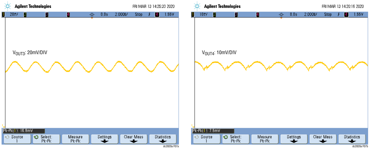
Figure 7. 12V IN Measured Output Ripple for V OUT3 = 1.5V and V OUT4 = 1.2V at 3A Load
