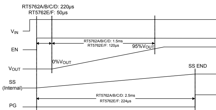
Figure 1. Start-Up Sequence
