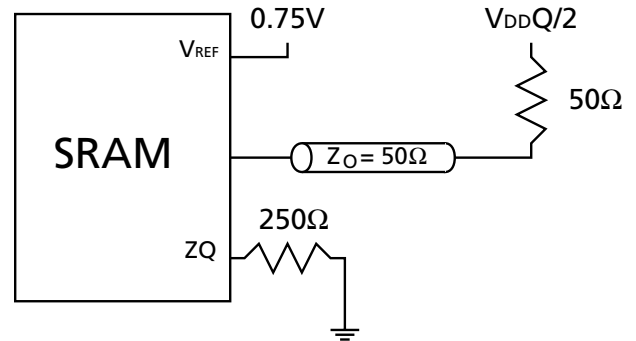
Figure 5: Output Load Equivalent
