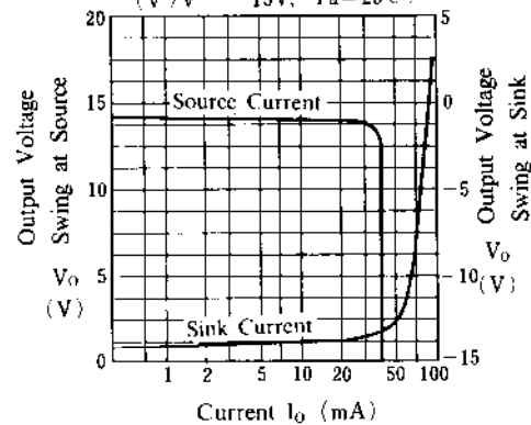
Output Source Current vs. Output Voltage Swing
