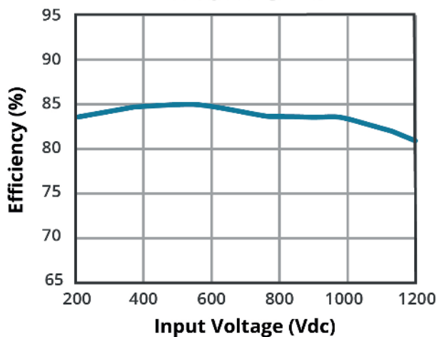
EFFICIENCY VS INPUT VOLTAGE AE40-EW-S12-T
