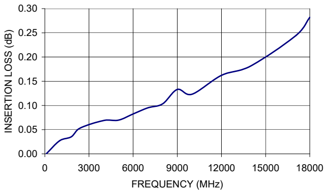
141-4SMR+ INSERTION LOSS
