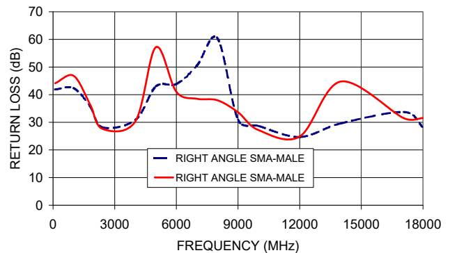
141-4SMR+ RETURN LOSS
