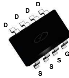
SOP-8
