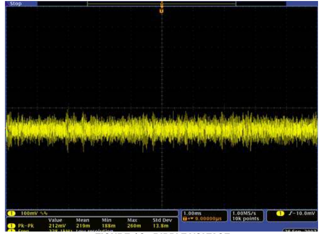
FIGURE 16. RIPPLE VOLTAGE
