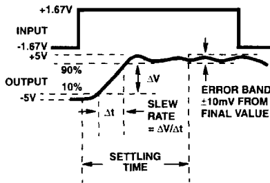
FIGURE 1. SLEW RATE AND SETTLING TIME
