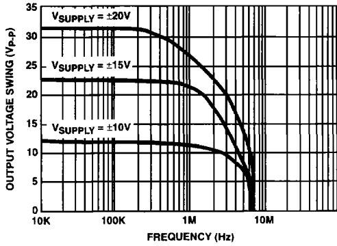
FIGURE 18. OUTPUT VOLTAGE SWING vs FREQUENCY
