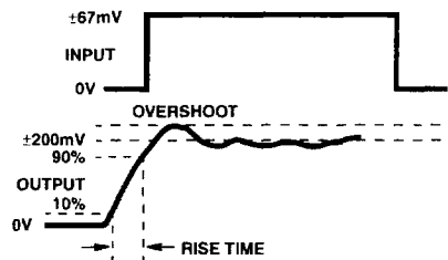
FIGURE 2. TRANSIENT RESPONSE
