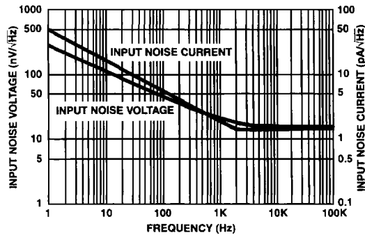
FIGURE 17. INPUT NOISE CHARACTERISTICS
