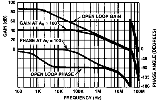
FIGURE 15. FREQUENCY RESPONSE
