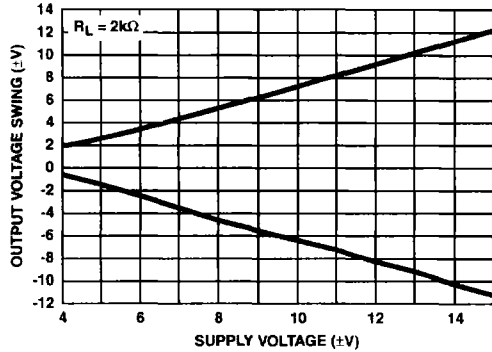
FIGURE 13. OUTPUT VOLTAGE SWING vs SUPPLY VOLTAGE
