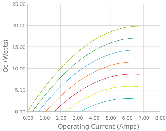
Heat Pumped at Cold Side T hot = 27 °C
