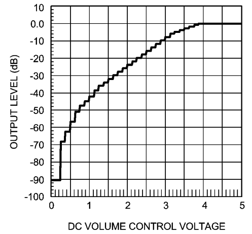
Volume Control Characteristics
