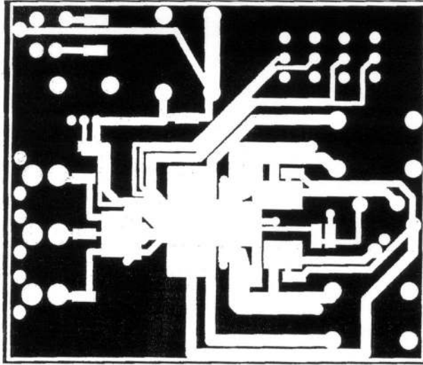
FIGURE 7. Inner Layer (2)
