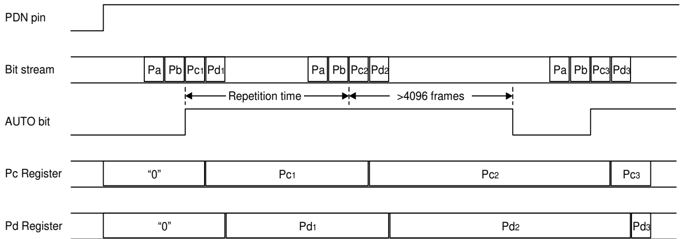
Figure 51. Timing example 1
