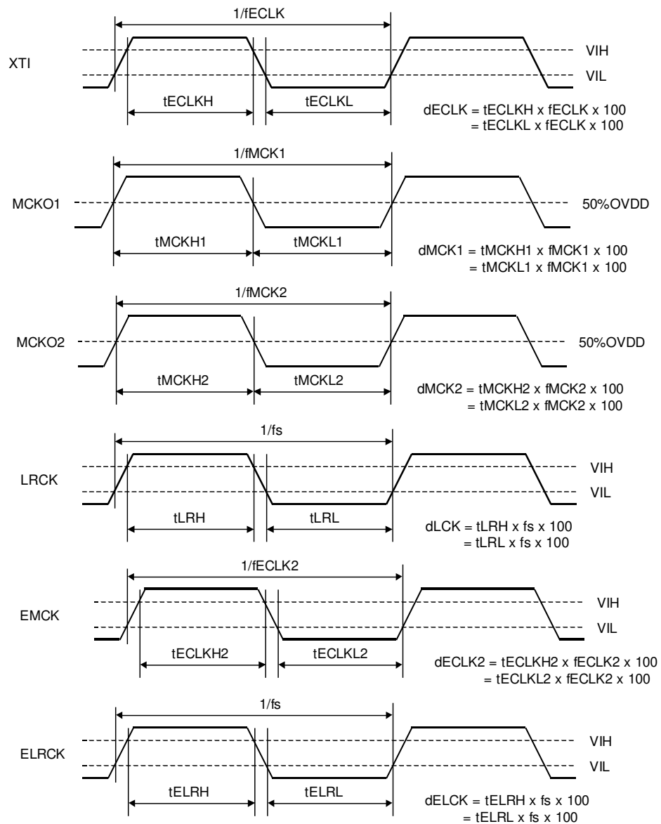
Figure 3. Clock Timing
