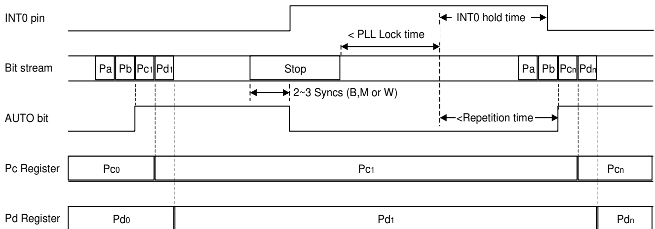
Figure 52. Timing example 2
