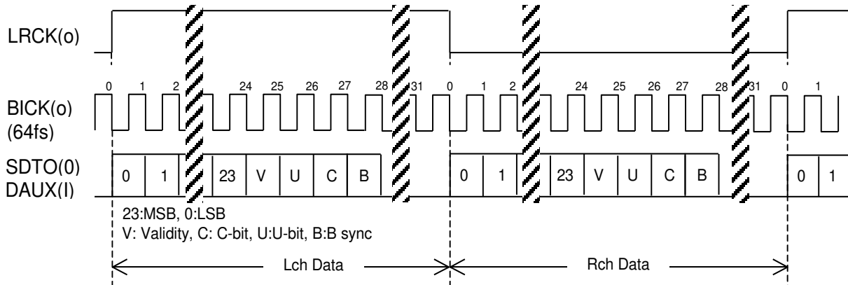
Figure 39. AES3 Mode
