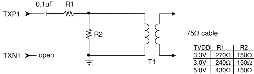
Figure 26. Consumer Output Driver Circuit at AC coupling
