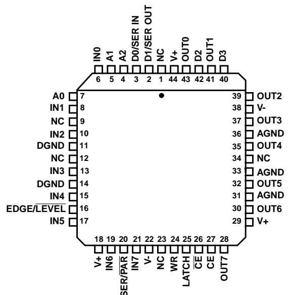
HA456 (PLCC) TOP VIEW
