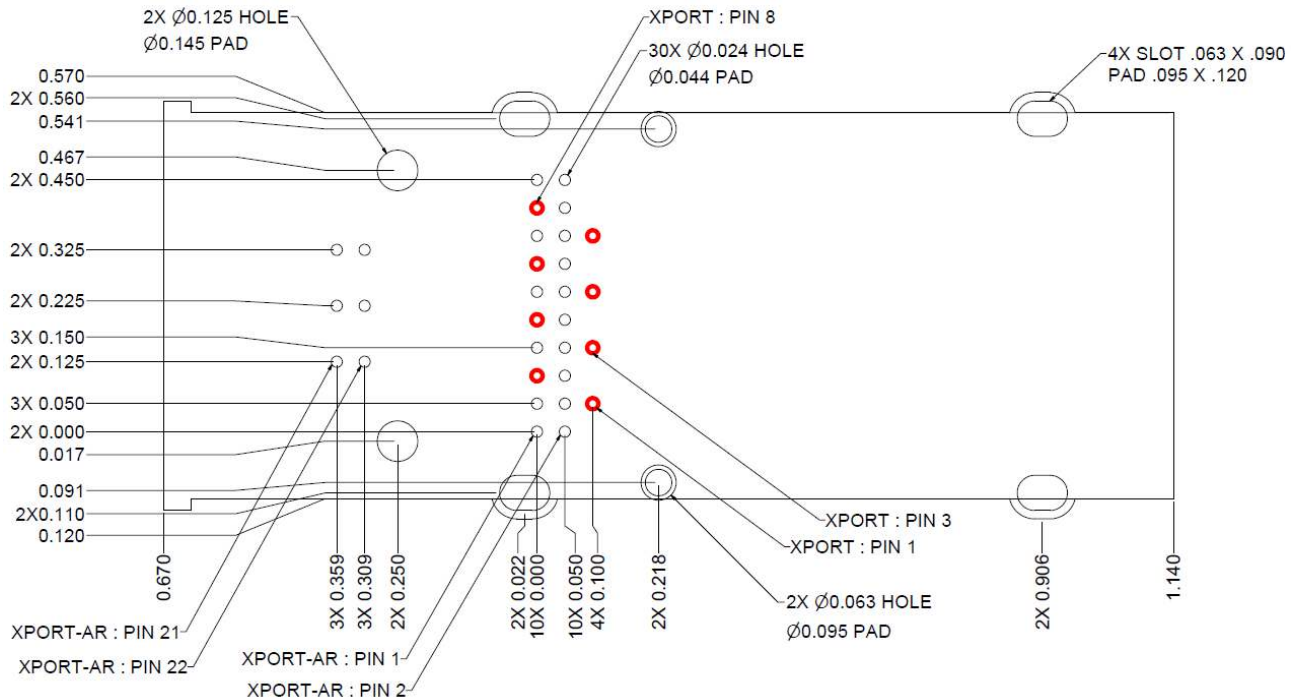
Figure 2-8. Hole Pattern and Mounting Dimensions (Bottom View)
