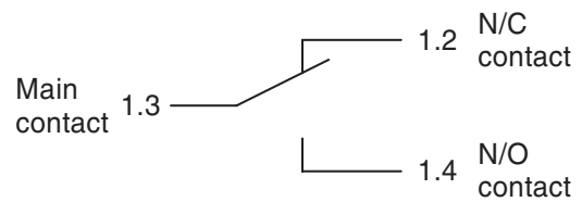
Figure 4 Output relay contacts
