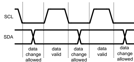
Figure 33. Data Validity
