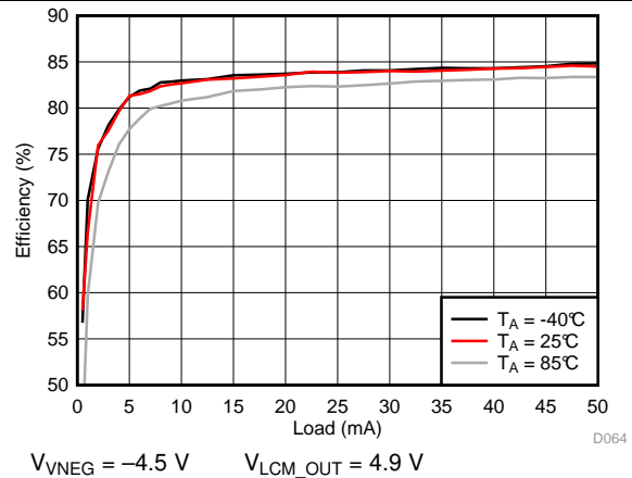
Figure 85. VNEG Efficiency
