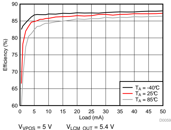
Figure 80. VPOS Efficiency
