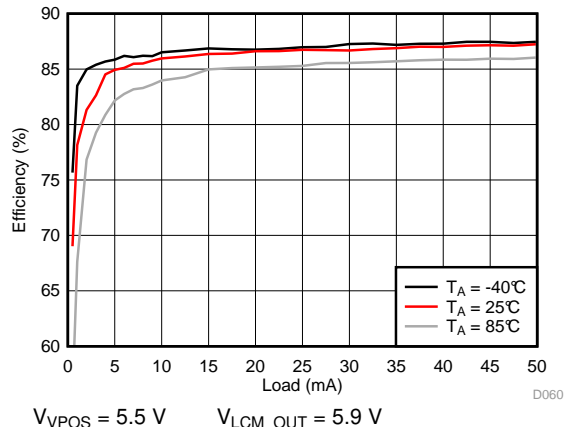
Figure 81. VPOS Efficiency
