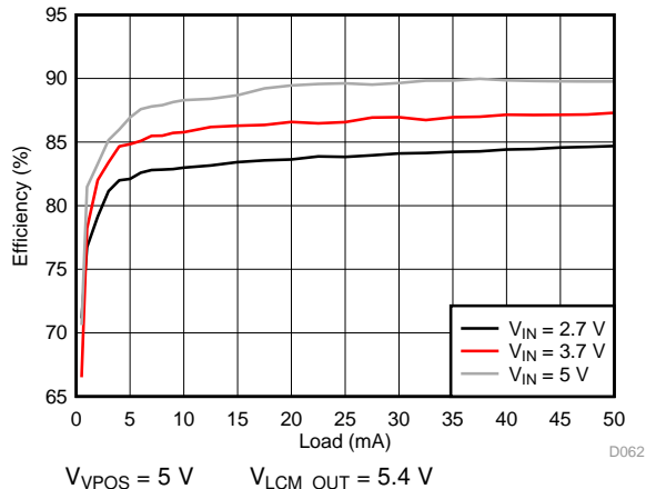
Figure 83. VPOS Efficiency
