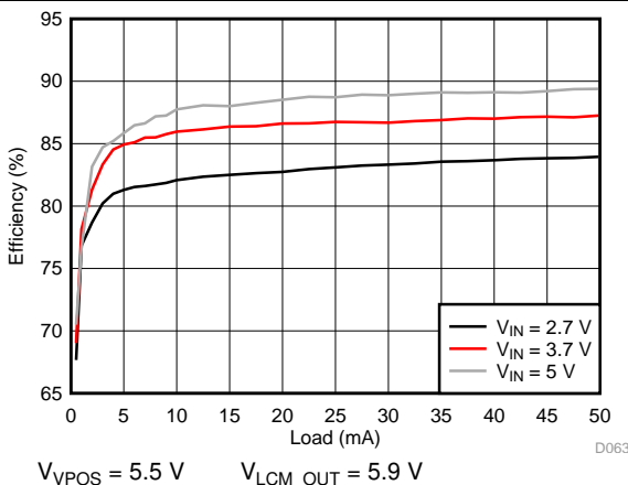
Figure 84. VPOS Efficiency
