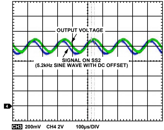
Figure 12. External Signal Tracking at 3 A Load
