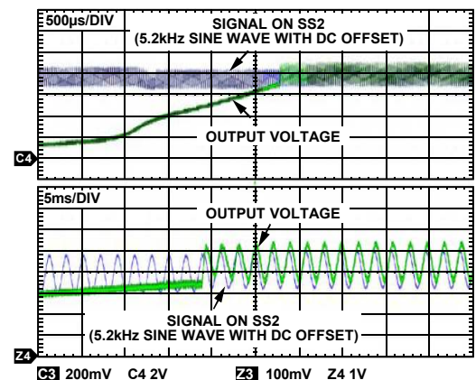
Figure 14. External Signal Tracking at 3 A Load During Start Up
