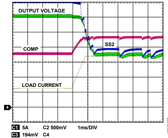
Figure 24. OCP Recovery During Load Step 6 A to 14 A
