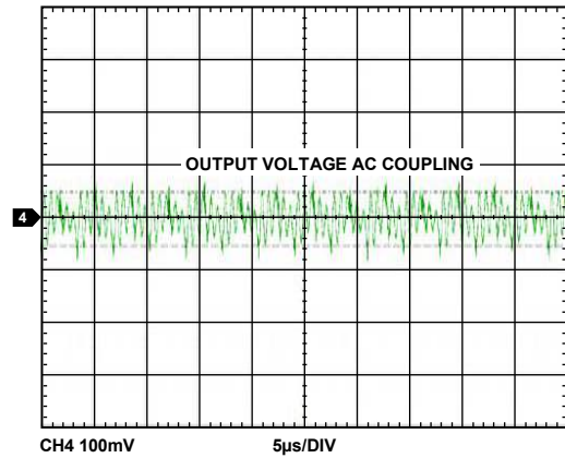
Figure 8. Output Ripple at 48 VDC Input, No Load
