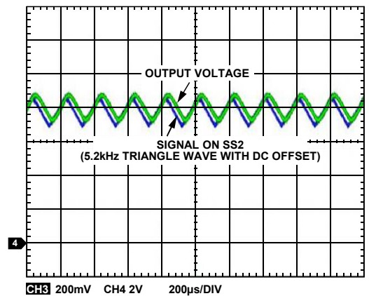
Figure 13. External Signal Tracking at 3 A load
