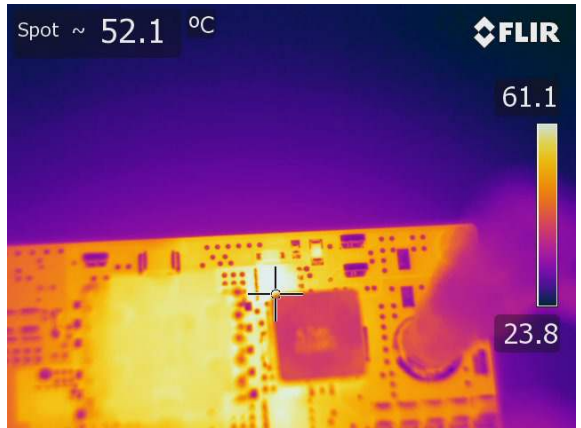
Figure 30. Thermal Image of SR1 at 48 V DC Input, 6 A Load, No Airflow, 1 Hour Soaking Time
