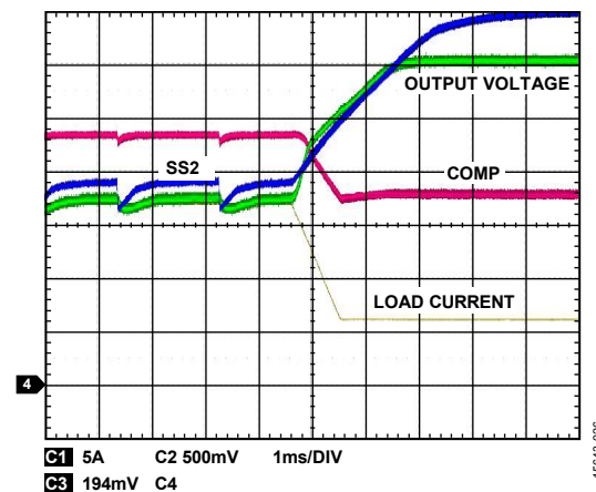
Figure 25. OCP Recovery During Load Dump, 14 A to 6 A
