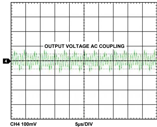
Figure 9. Output Ripple at 48 VDC Input, 6 A Load
