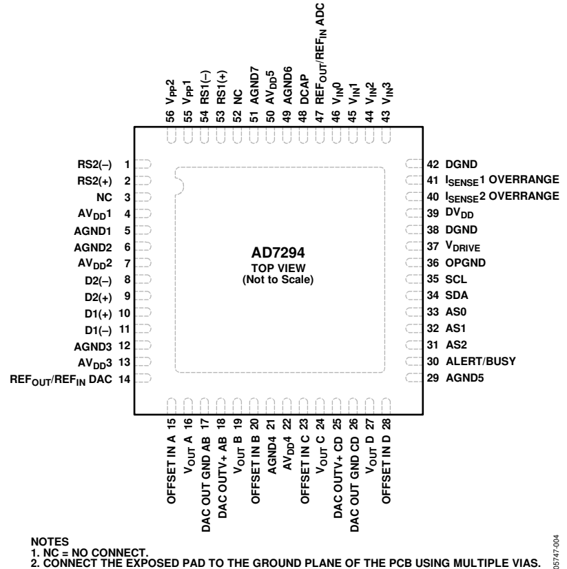
Figure 5. LFCSP Pin Configuration
