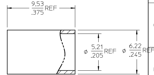
CRIMP TUBE
