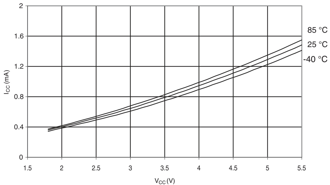
Figure 31-294. ATmega328: Idle Supply Current vs. V_{CC} (Internal RC Oscillator, 8MHz)
