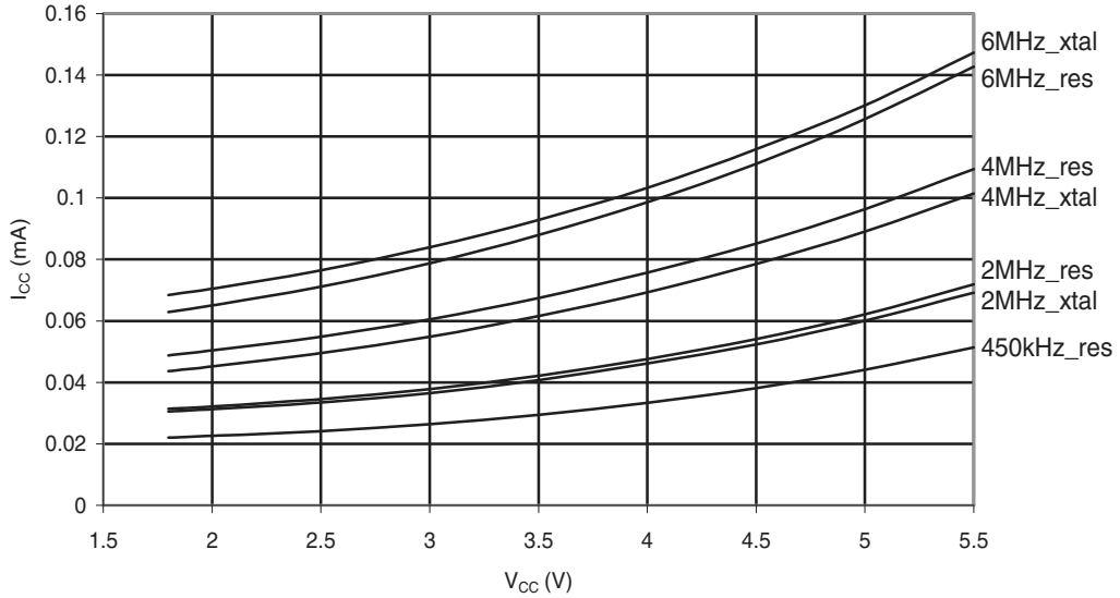
Figure 31-14. ATmega48A: Standby Supply Current vs. V_{CC} (Watchdog Timer Disabled)
