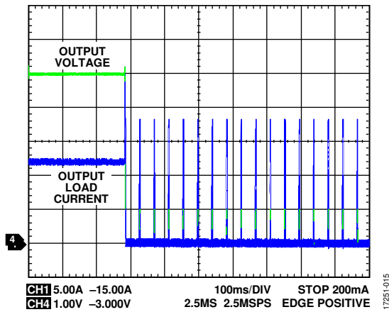
Figure 14. Overcurrent Protection, 100 ms/div
