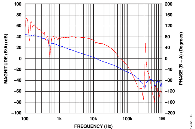
Figure 12. Loop Gain Measurement by the AP200 Loop Analyzer with R18 = 49.9 kΩ; 12 V Input, 12 A Load; Crossover Frequency = 11.79 kHz, Phase Margin = 54.2°, Gain Margin = 17.9 dB
