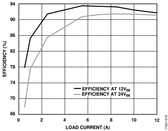
Figure 18. Efficiency Curves
