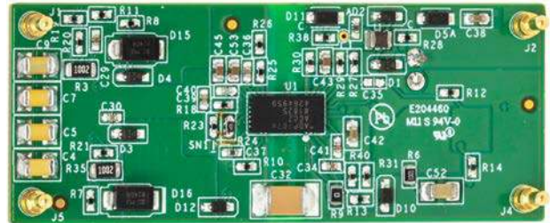
Figure 4. ADP1074 LGA-EVALZ Evaluation Board, Bottom Side
