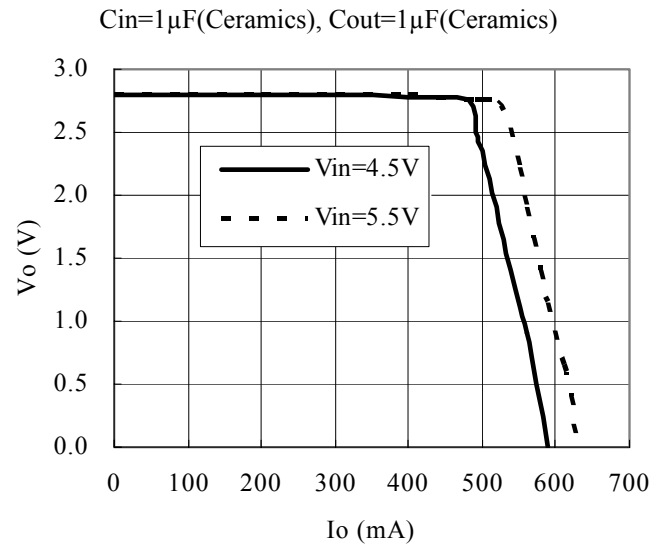
PT7M8202 (3.3V)
