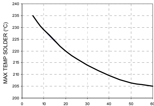
Figure 19. Time Limit Curve Above 205°C for Tin/Lead (Sn/Pb) process.
