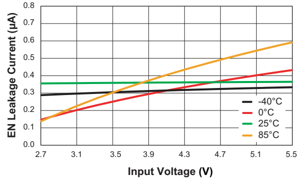
EN Leakage Current vs. Input Voltage
