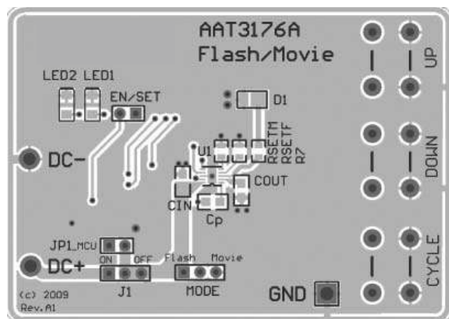
Figure 4: AAT3176A Evaluation Board Layout Top Layer.
