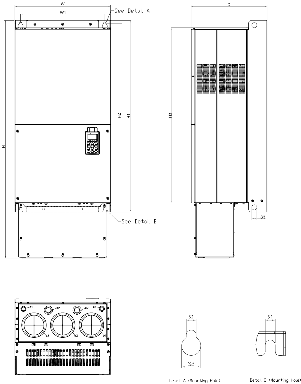
Detail A (Mounting Hole)
