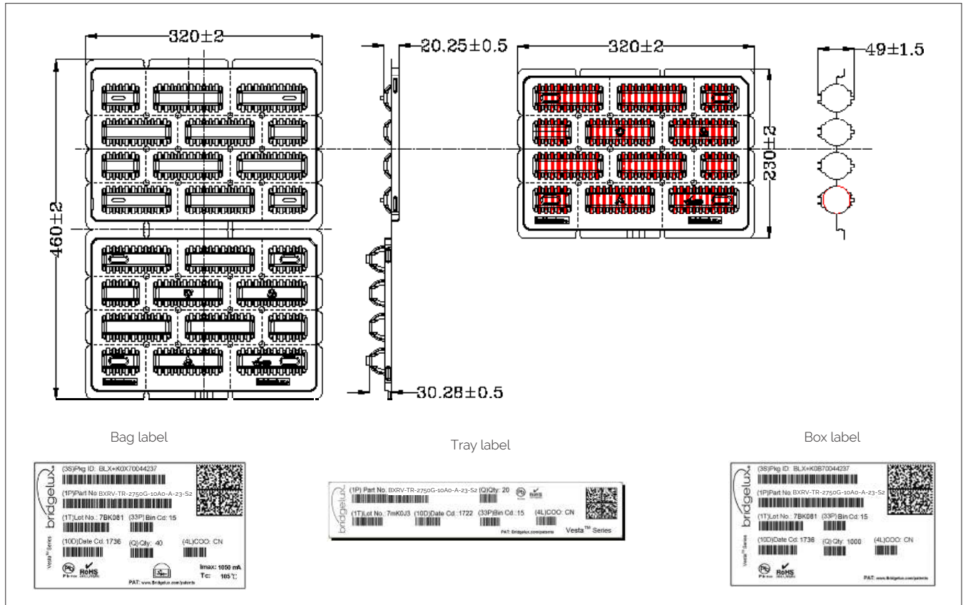
Figure 40: Packaging Specifications
