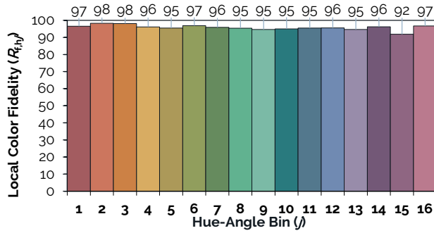
Figure 3: 6500K Thrive TM-30 Graphs
