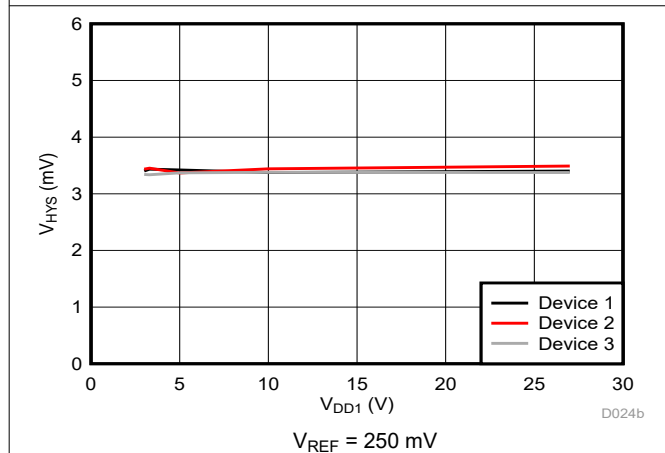
Figure 6-15. Trip Threshold Hysteresis vs Supply Voltage
