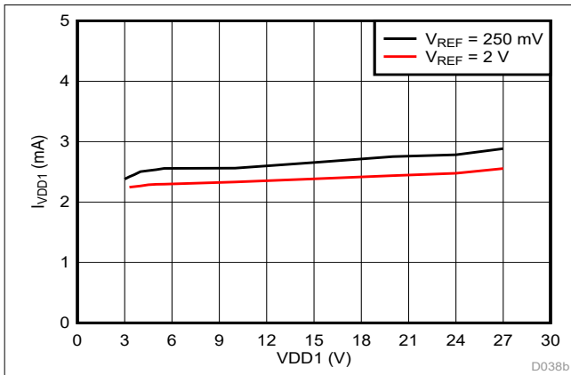
Figure 6-29. High-Side Supply Current vs Supply Voltage
