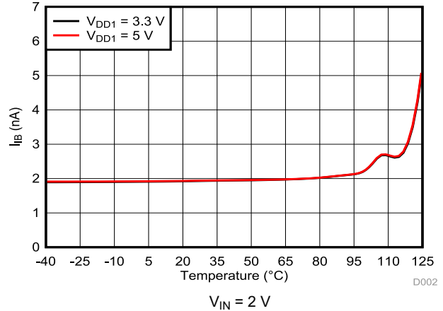
Figure 6-26. Input Bias Current vs Temperature
