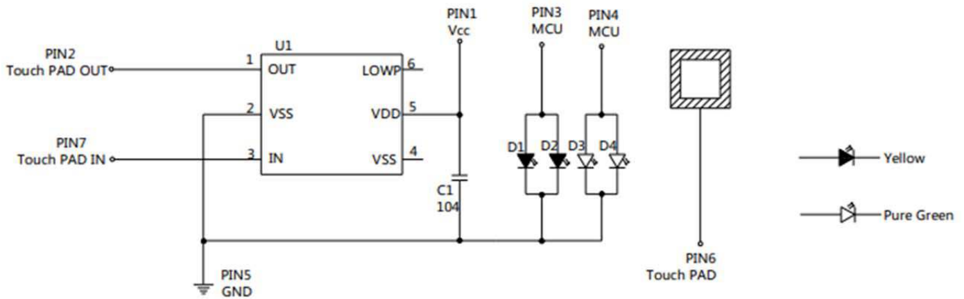
PIN 7 Layout connection to PIN 6
