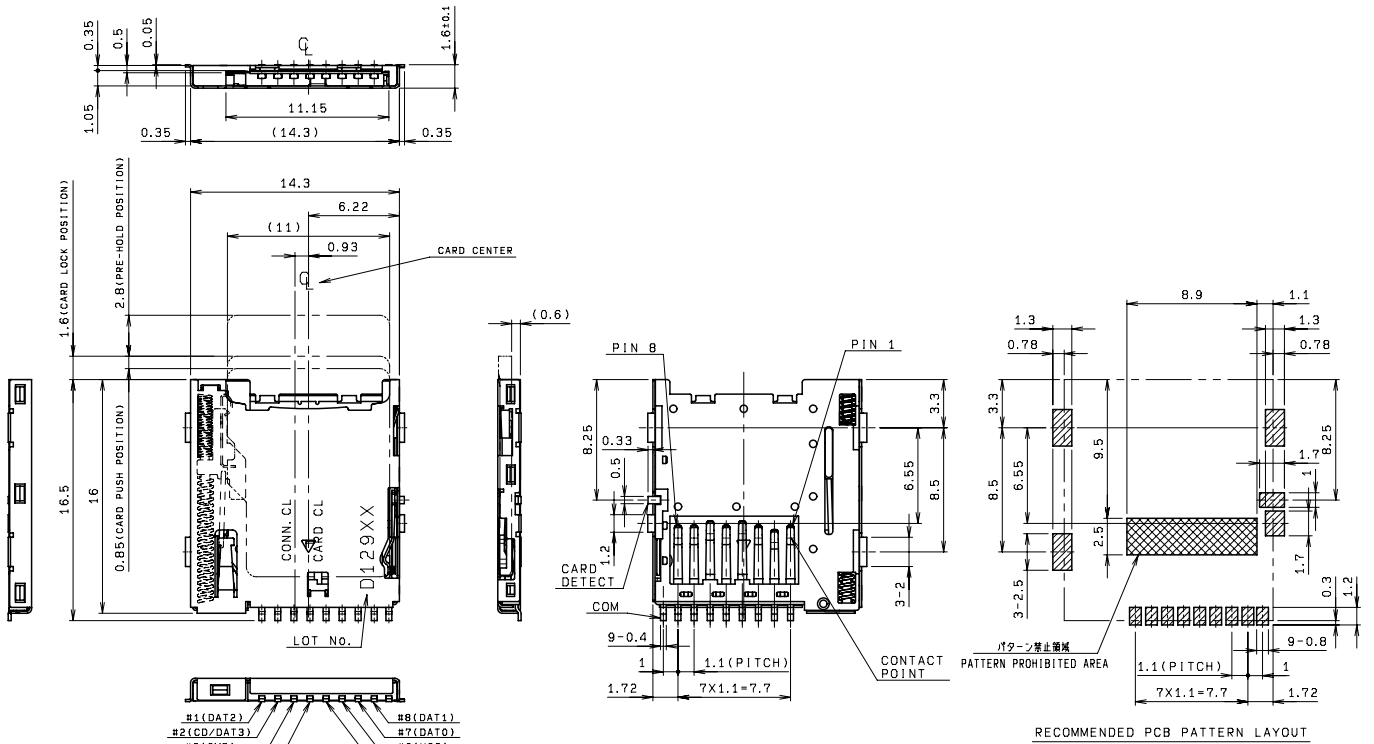
RECOMMENDED PCB PATTERN LAYOUT
