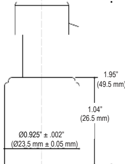
Metri-Pack 150 Series
