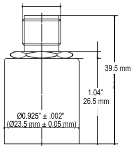
M12 X 1 (4-pin)
