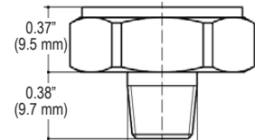
1/8" NPT Male
