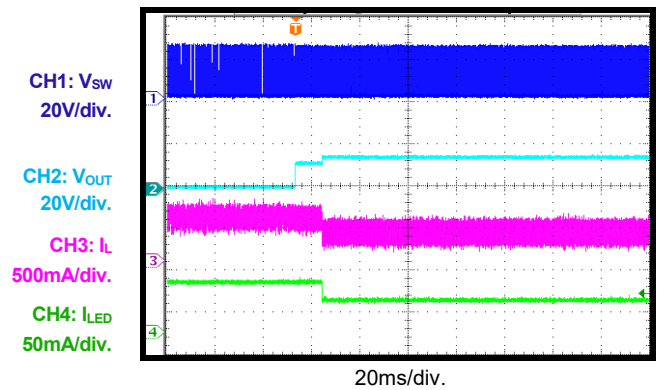
Short LED Protection (Marked Off)
