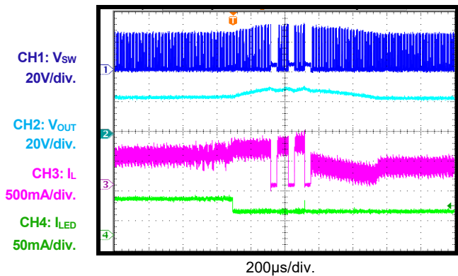
Open LED Protection (Marked Off)
