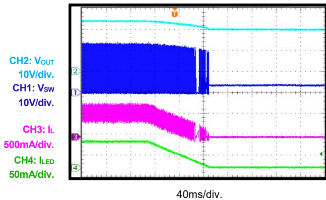
En Bit Off 62.5 \mu s/step
