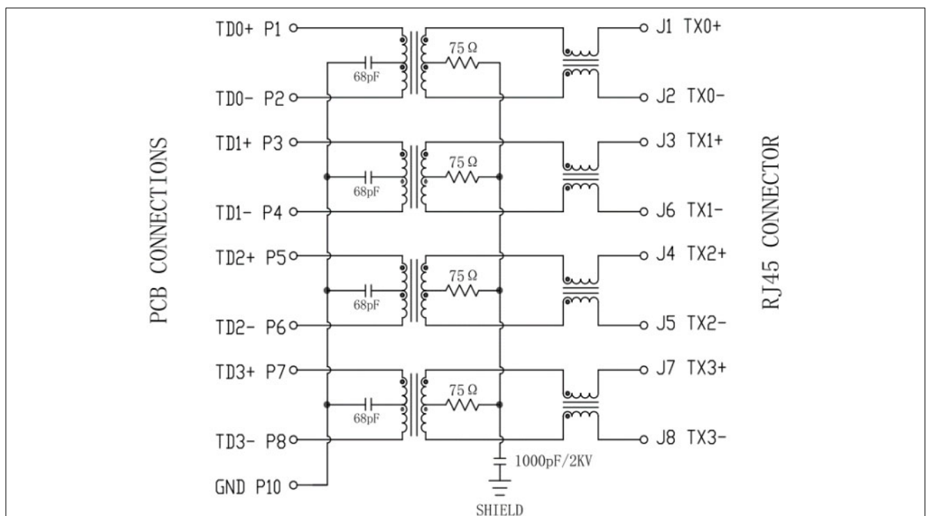
Figure 57 Schematic of a Transformer with CMC on Line
