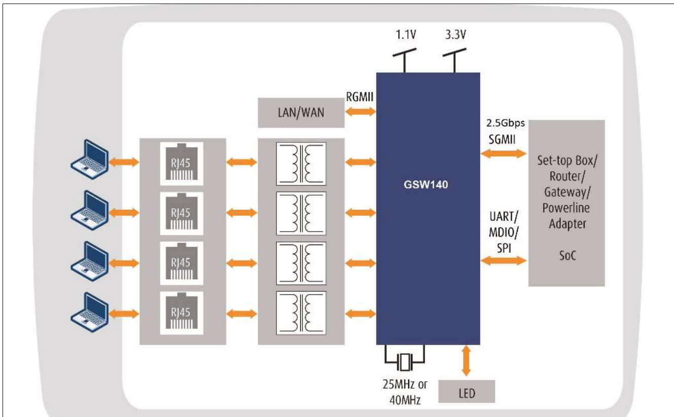
Figure 3 Home Gateway
