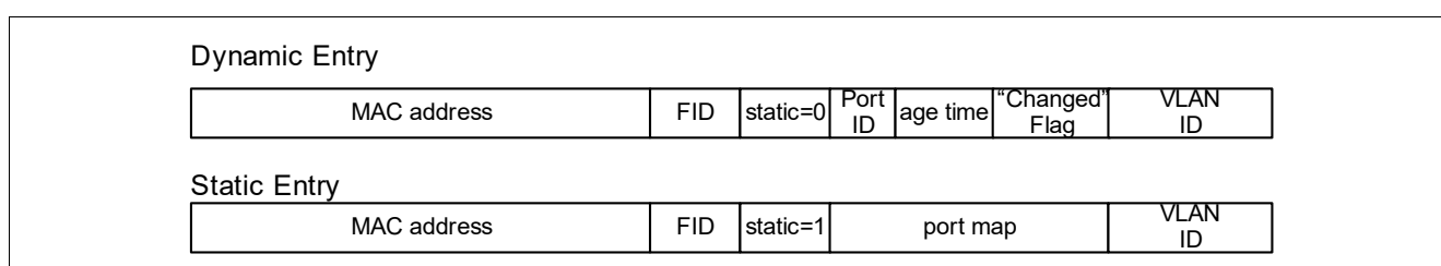
Figure 27 MAC Bridge Table Entry Formats
