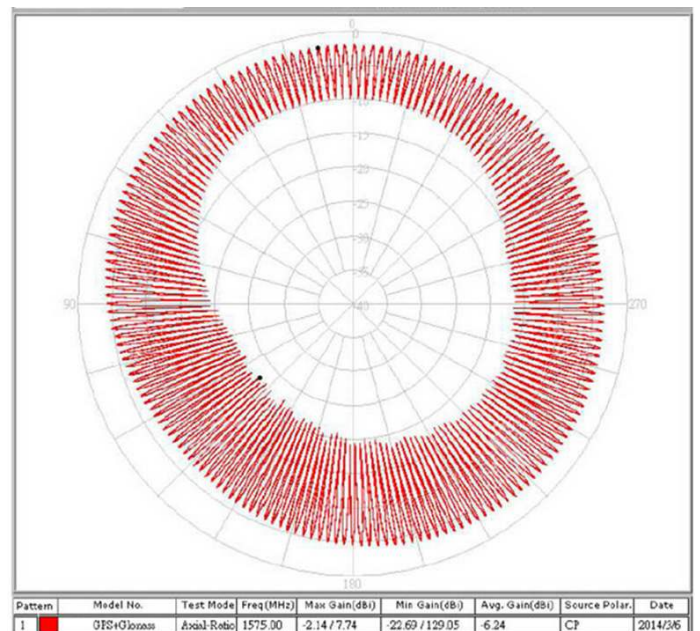
Axial Ratio@1575MHz
