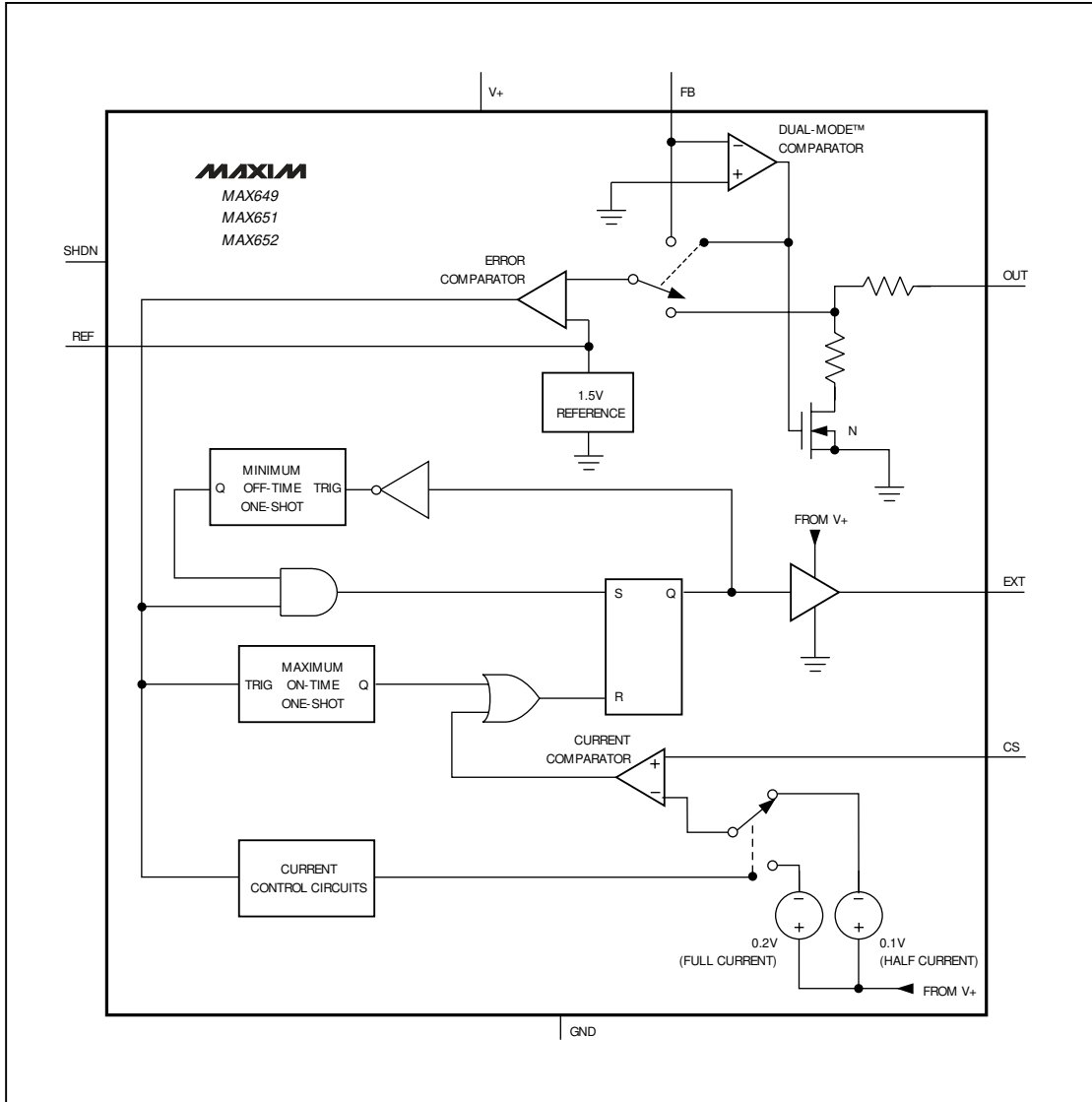
Figure 2. Block Diagram
