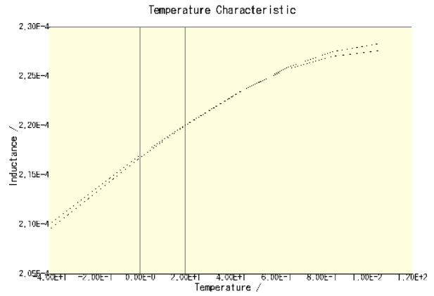
CLF12555T-221M-CA(DC = 0A)
