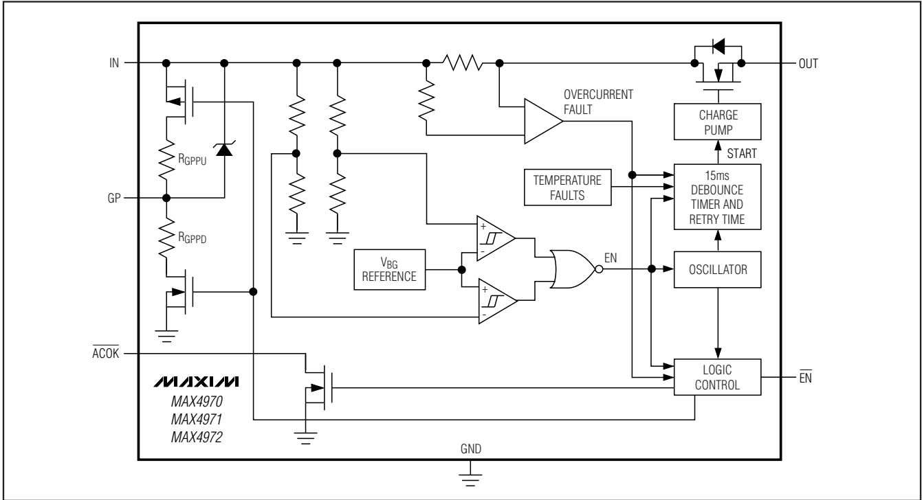
Functional Diagram
