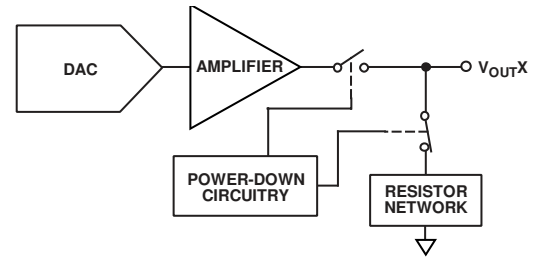
Figure 52. Output Stage During Power-Down
