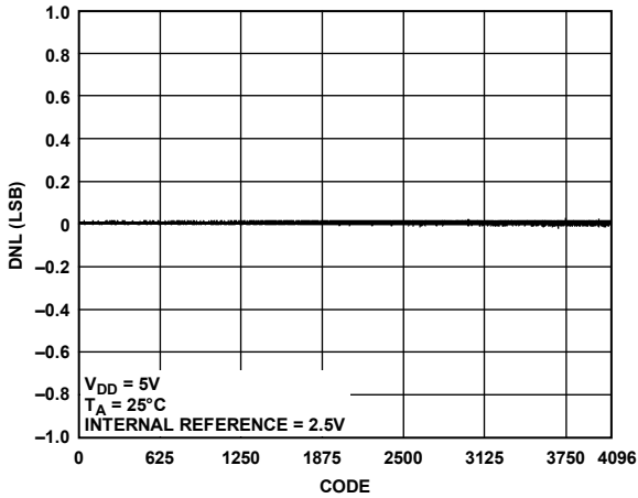
Figure 17. AD5694R DNL
