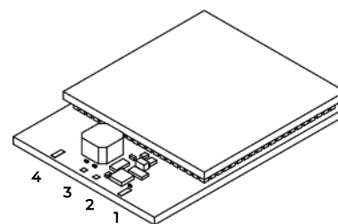
Figure 4. Pinouts for PRMT**-34465-***
