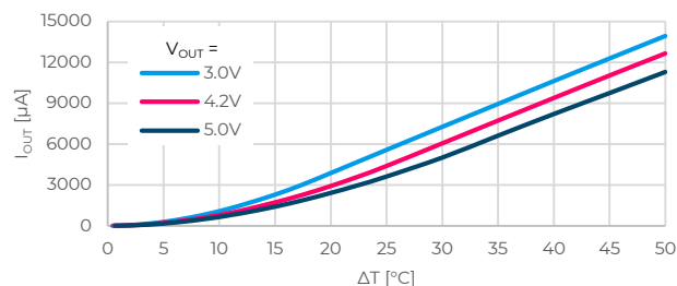
Figure 13. Output current for PRMT02-34465-**B with 1/K_{TEG}=2K/W
