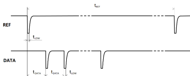
Figure 14. Timing charts of ADC Outputs
